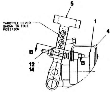
VIEW A-A ITEMS #2, 23 & 27 NOT SHOWN FOR CLARITY
